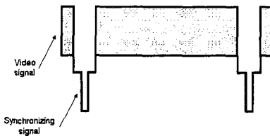
Figure 5-13(a) (┐┘) Sync signal
