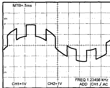
Figure 5-6 Typical ADD waveform
